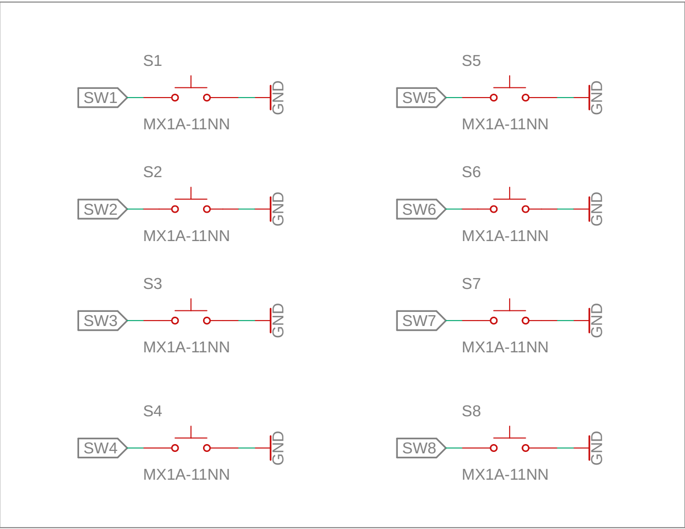
Switch Matrix
