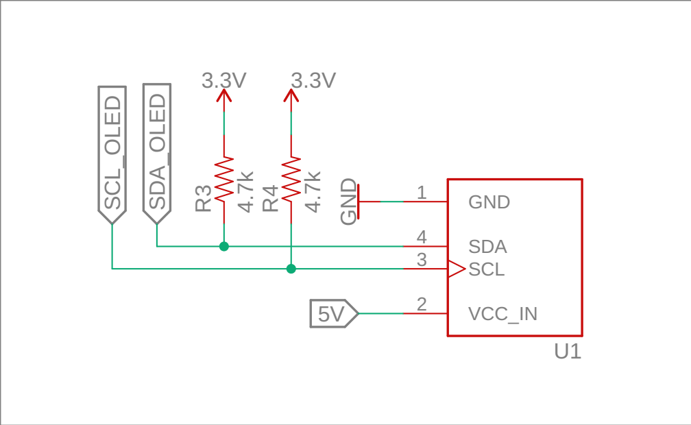
DM-OLED096-636 OLED Display
