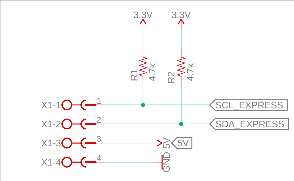
PHOENIX_508_4PIN connection to ItsyBitsy m0 Express
