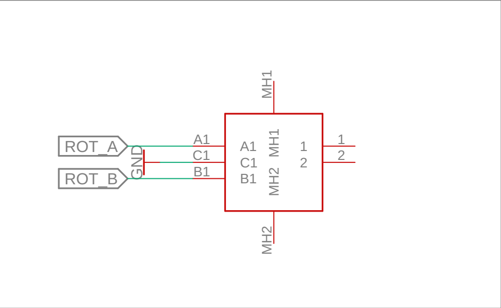
PEC11L-4115F-S0020 Rotary Encoder
